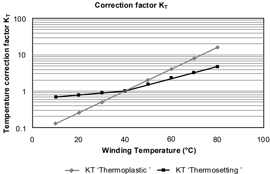
Figure 5 —Temperature correction factors for “THERMOPLASTIC” (asphaltic) and “THERMOSETTING” (epoxy or polyester) insulation systems
